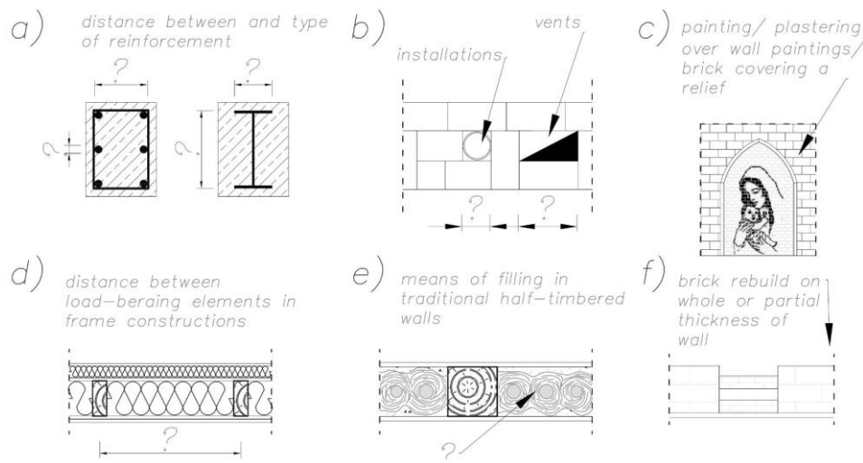
Fig. 1. Examples of applying active thermography in studies on historic buildings
