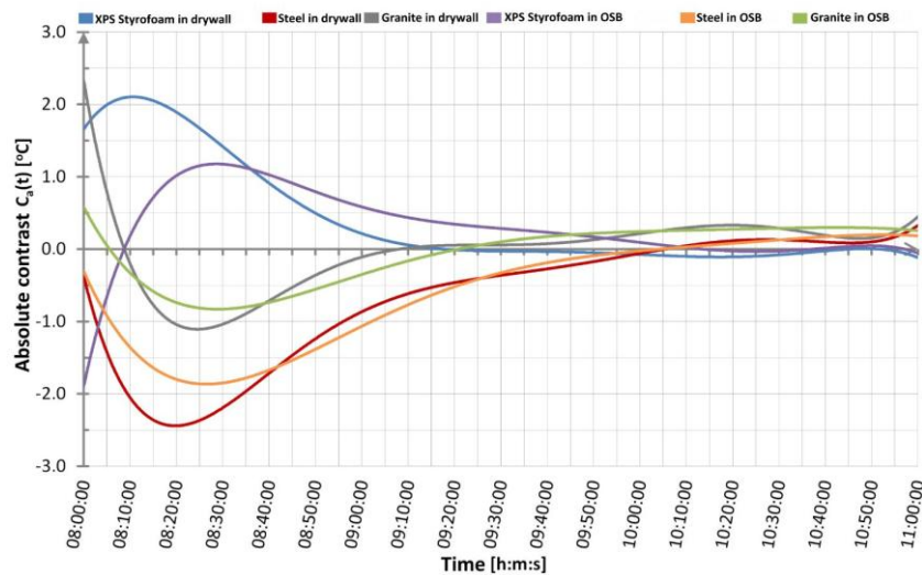
Fig. 3. Values of absolute contrast during the cooling of the analyzed surface (description in text)
