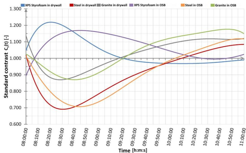
Fig. 4. The value of standard contrast during the cooling of the analyzed surface (description in text)
