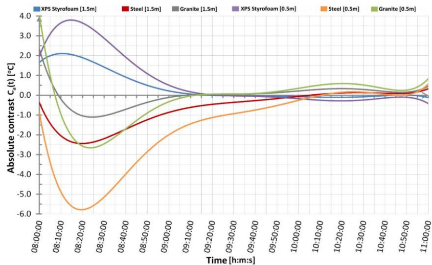
Fig. 5. Differences absolute contrast at two different levels of heating the surface (temperatures provided in the legend)
