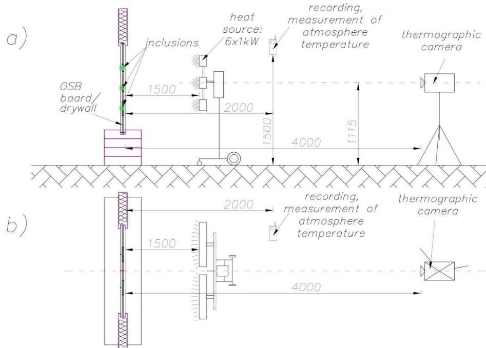
Fig. 2. Plan of test station applied in active thermography in the reflective mode
