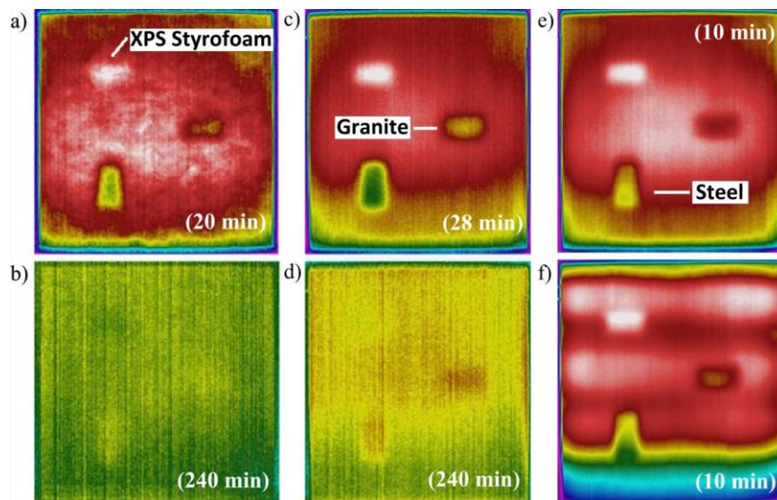
Fig. 6. Thermograms for models of OSB board (a, b), drywall (c, d), and various degrees of heating the surface (e, f); the time from when the heat source was turned off has been provided in the brackets
