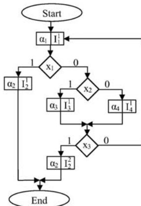
Fig. 3. OLC flow-chart of the CMCU U_1 .
